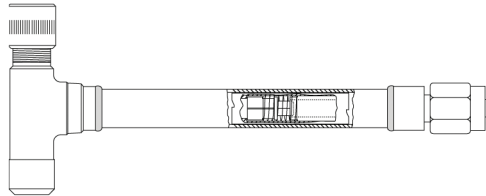
Model 13 — Steel tee with Model 35 installed
